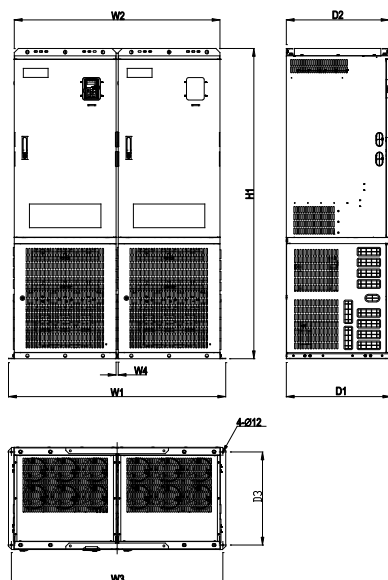
Figure 2-6 Parallel installation dimension for 380V 710–3000kW and 660V 800–3600kW models
