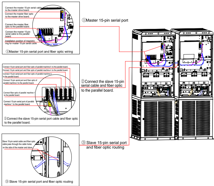
Figure 3-4 Master-slave connection diagram 1 (710–3600kW)
